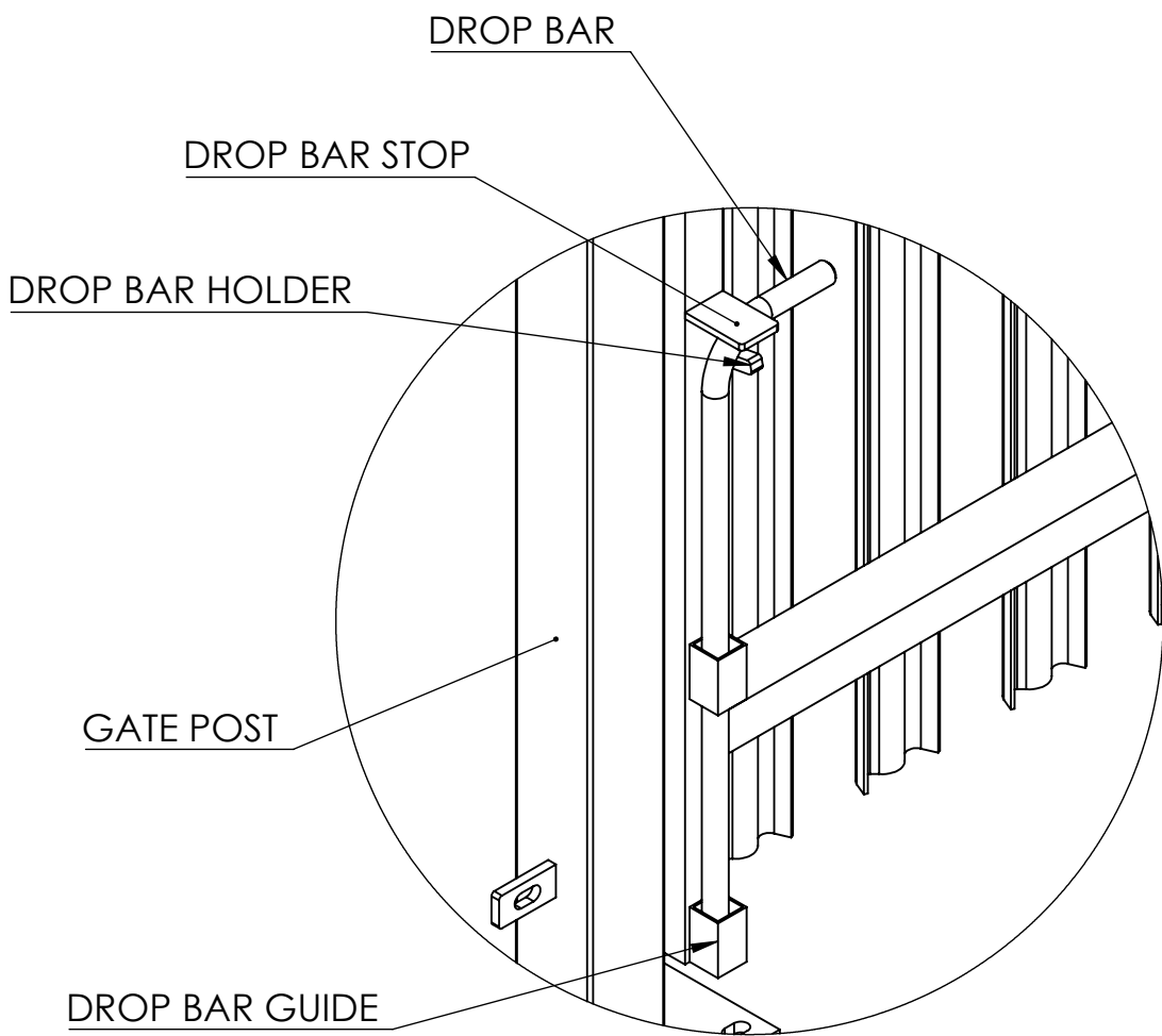
Back View of Drop Bar & Guides
