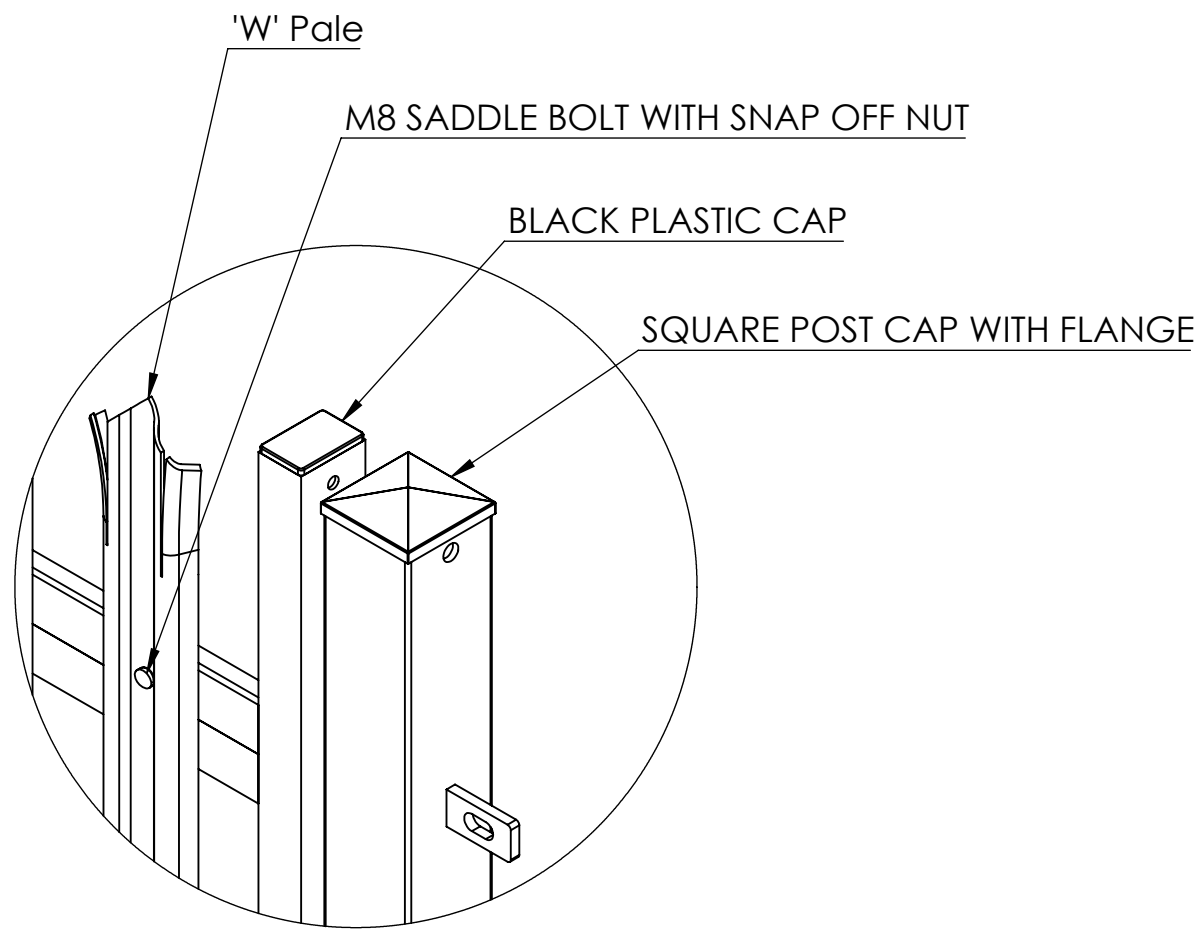
Gate & Post Attachment Example
