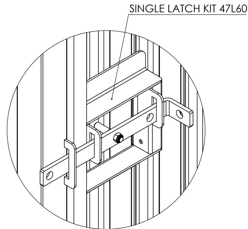
Slide Latch With Padlock Holes & Reversible Handle As Standard. (Padlock Not Included)
